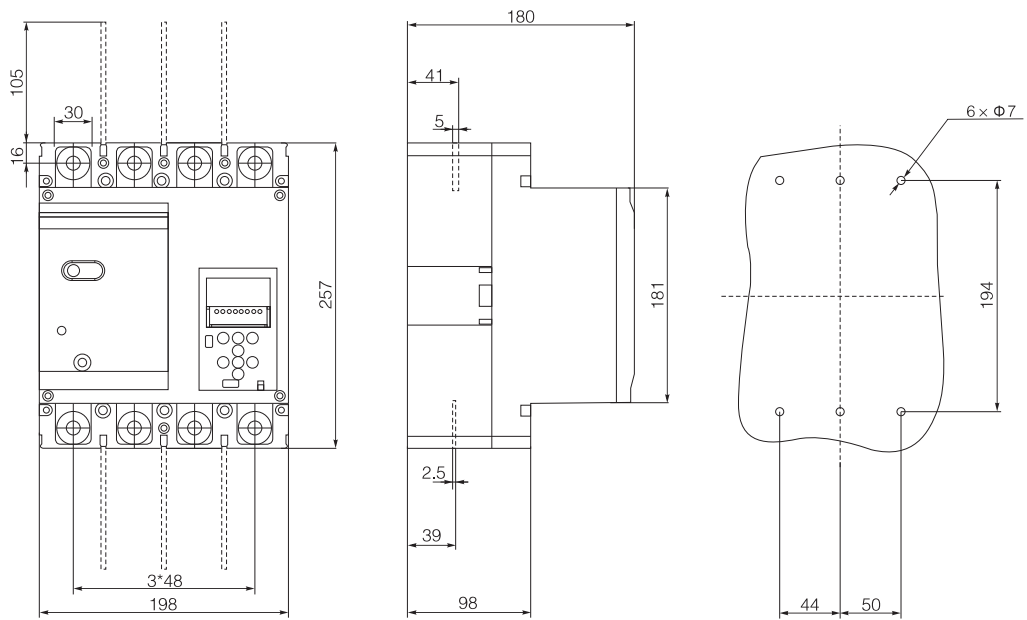
图2 CFM8LC-400
