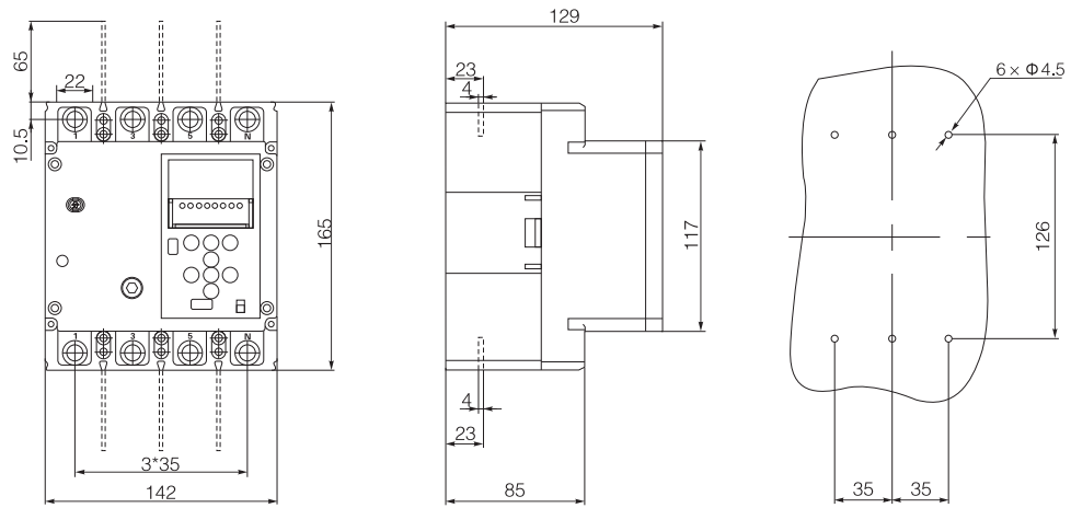
图1 CFM8LC-250
